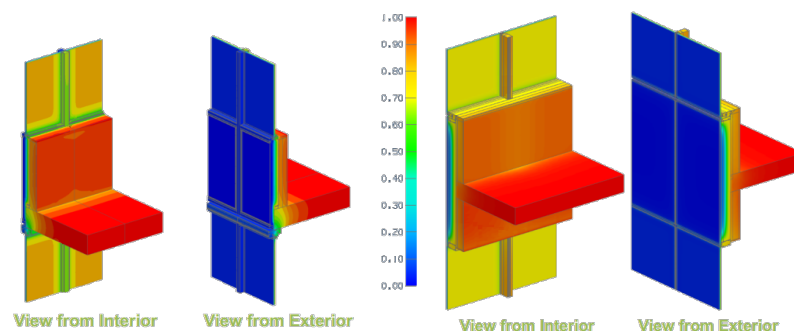
Figure 3: Thermal Gradients of Window Wall and Curtain Wall (Morrison Hershfield, 2016)
