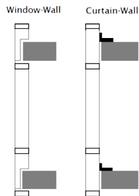
Figure 2: Simplified Window Wall and Curtain Wall
