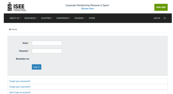
Figure 1: Login Page
