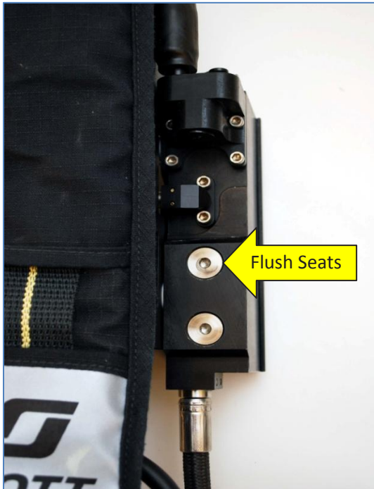
Figure 1 - Air-Pak 75 without adjustable seats
