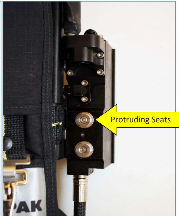
Figure 2- Air-Pak 75 WITH adjustable seats SUBJECT OF THIS NOTICE
